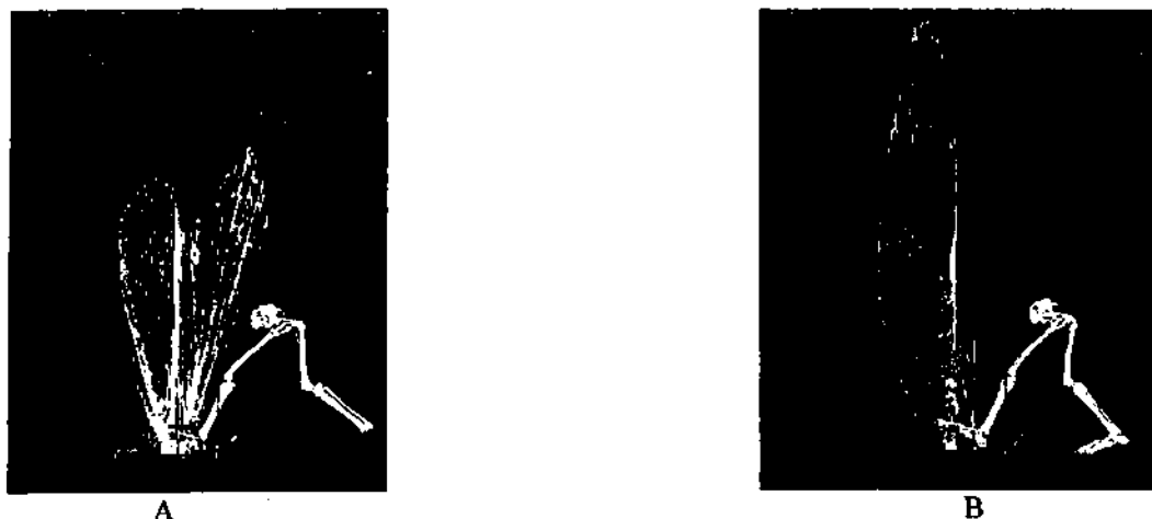
Fig. 3. Vector plot of resultant support reaction when walking by the method of repulsion (A) and attraction/repulsion (B) [3]
